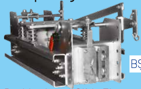
Double -Layer Slide Elevator Suspension Safety Gear
